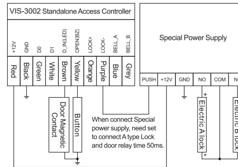
Wiring Diagram (Special Power Supply)
