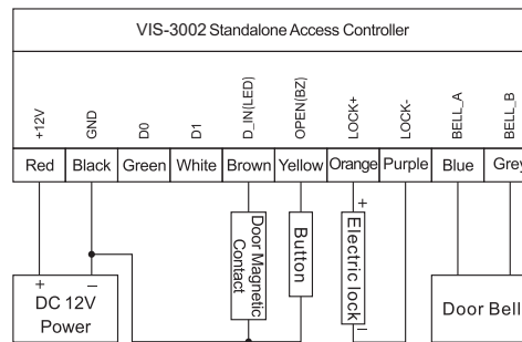
Wiring Diagram (DC Power Supply)
