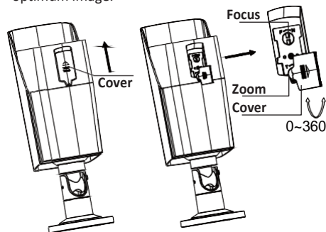
Figure 2-9 Zoom and Focus Adjustment
