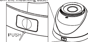
Figure 2-2 Release the Lock Screw
