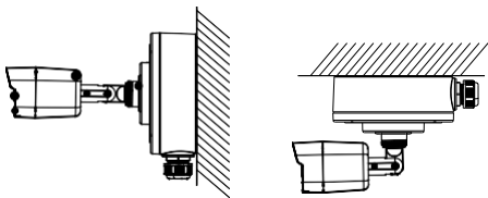
Figure 2-5 Fix the Camera to the Ceiling/Wall
