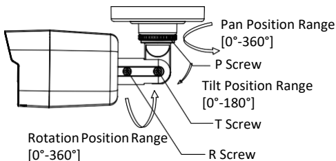
Figure 2-2 3-axis Adjustment
