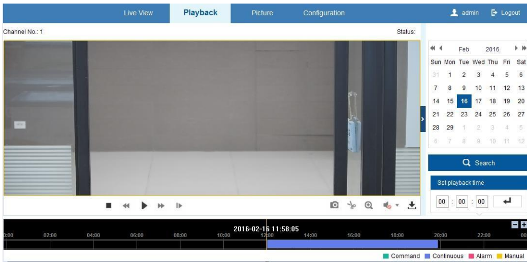
Figure 12-1 Playback Interface
