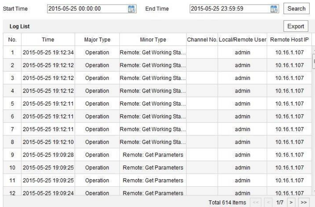
Figure 6-10 Log Searching
