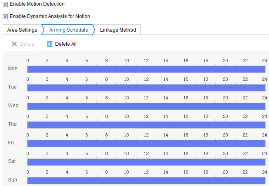
Figure 10-2 Arming Schedule
