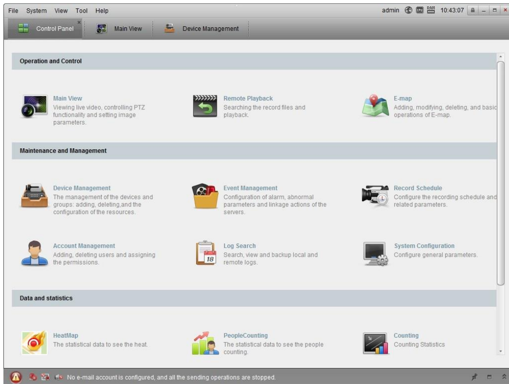
Figure 2-6 Control Panel
