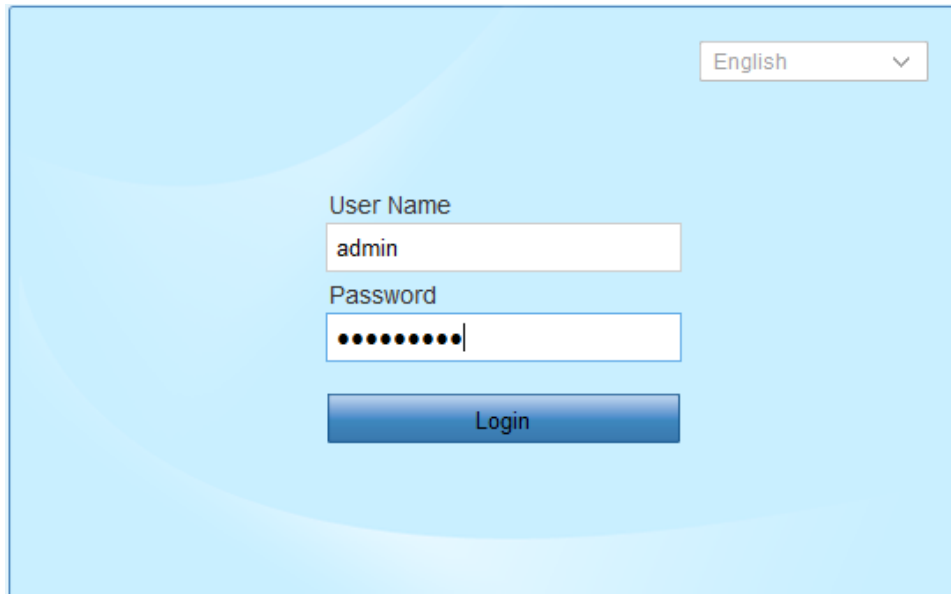
Figure 3-1 Login Interface
