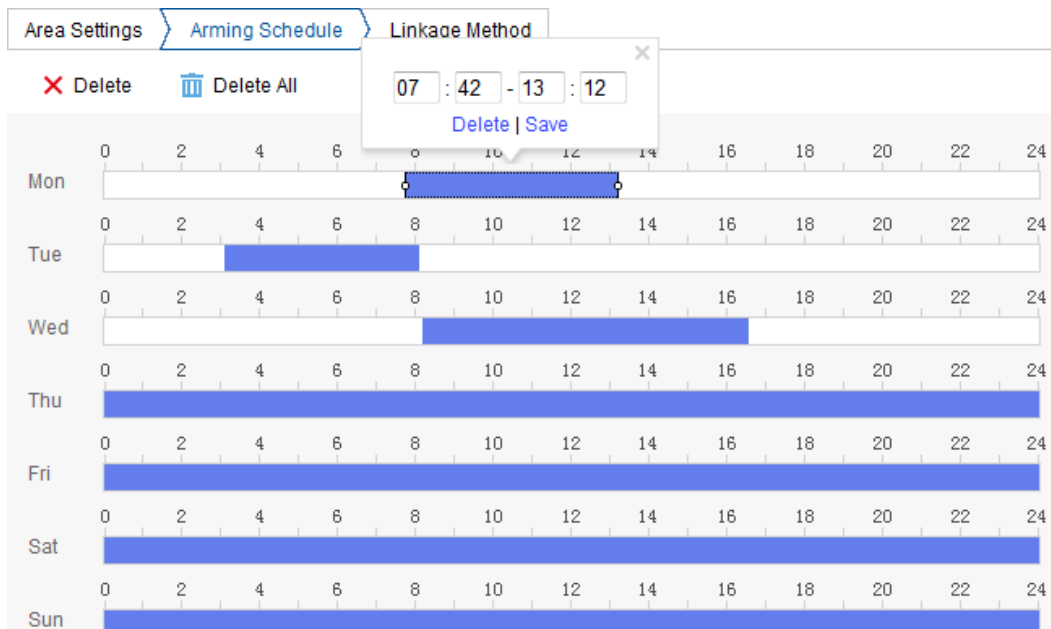
Figure 10-3 Arming Schedule
