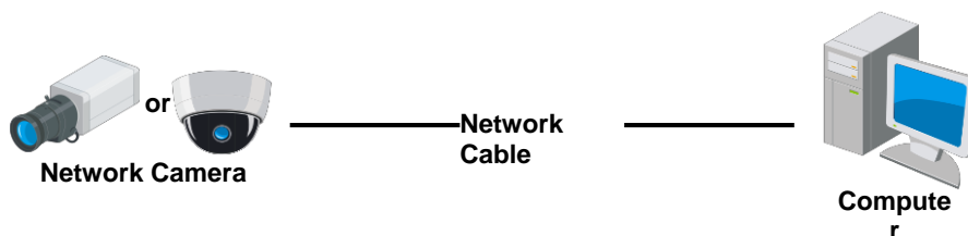
Figure 2-1 Connecting Directly
