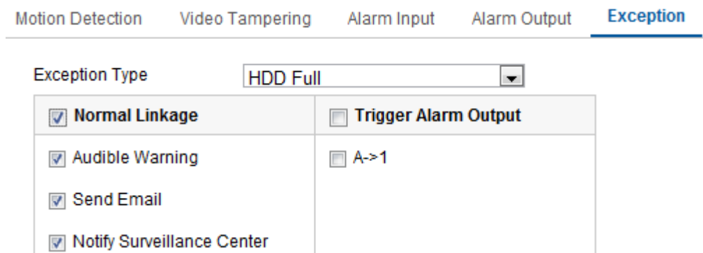
Figure 10-10 Exception Settings
