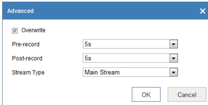
Figure 11-2 Record Parameters
