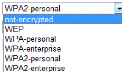
Figure 4-5 Security Mode
