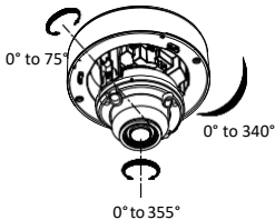
Figure 2-4 3-axis Adjustment
