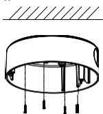
Figure 2-2 Attach the Back Box/Base Plate
