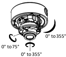
Figure 2-4 3-axis Adjustment
