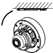
Figure 2-3 Fix the Camera to the Ceiling
